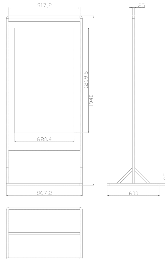
TECHNICAL DRAWING - 55" DISPLAY
